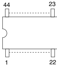
BD5422EFS-E2
