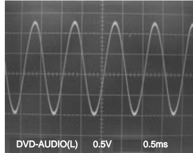
WF11 Pin 9 of CN201
