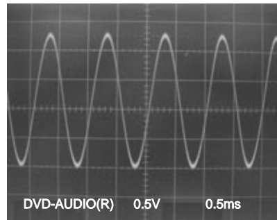
WF12 Pin 11 of CN201
