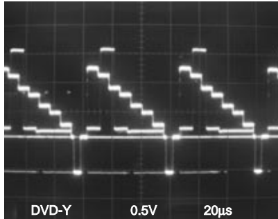
WF8 Pin 5 of CN201
