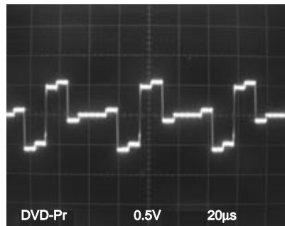
WF10 Pin 1 of CN201
