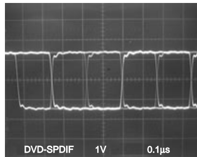
WF13 Pin 13 of CN201
